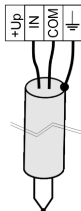
Thermocoupler
